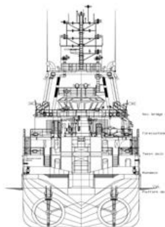
AFT VIEW
